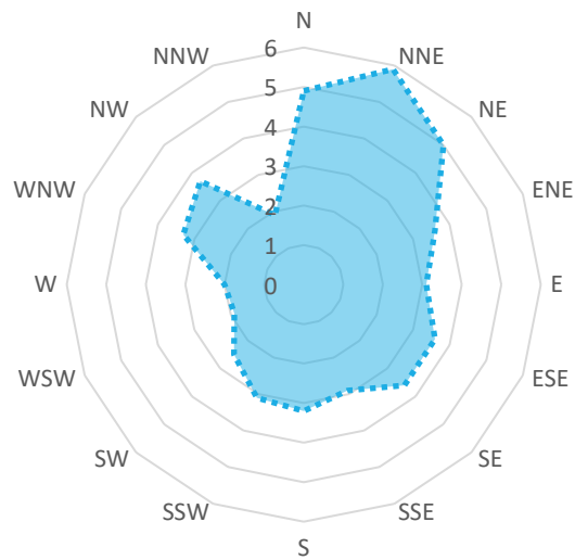
FIGURE 13. GWC JULY 2017 – JUNE 2018 AVERAGE WIND SPEED
