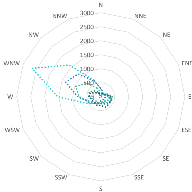
FIGURE 12. GWC JULY 2017 – JUNE 2018 WIND ROSE
