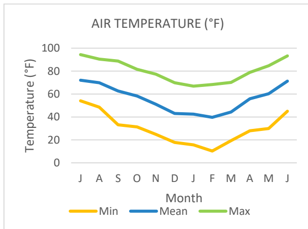
FIGURE 16. GWC JULY 2017 – JUNE 2018 AIR TEMPERATURE
